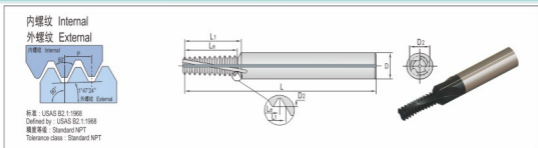
螺旋槽带内冷道孔螺纹铣刀 Helical Flutes with Thru-Hole Coolant
