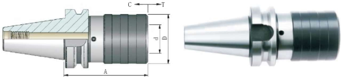
BT-弹性快换攻丝刀柄
