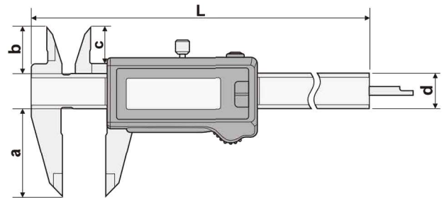
无内置发射 Without wireless data output
